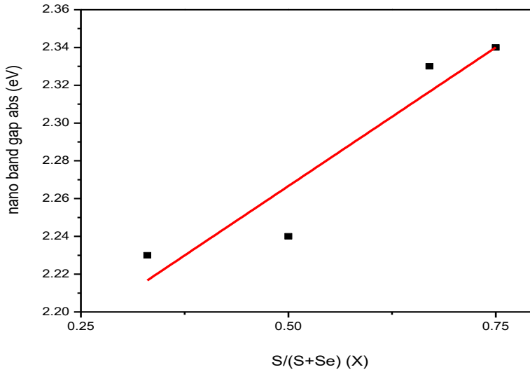
Fig. (4): shows the variation of nanocrystals bandgap energy with different S concentration
