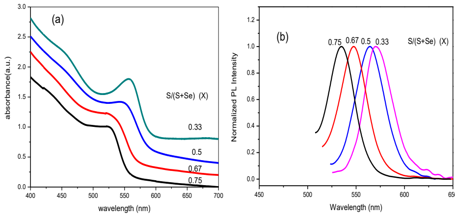
Fig. (3): UV-Vis absorption spectra (a) and PL spectra (b) of the CdS_xSe_{1-x} nanocrystals with different ratios (a) x = 0.33 , (b) x = 0.50 , (c) x = 0.67 and (d) x = 0.75 (S/S+Se).
