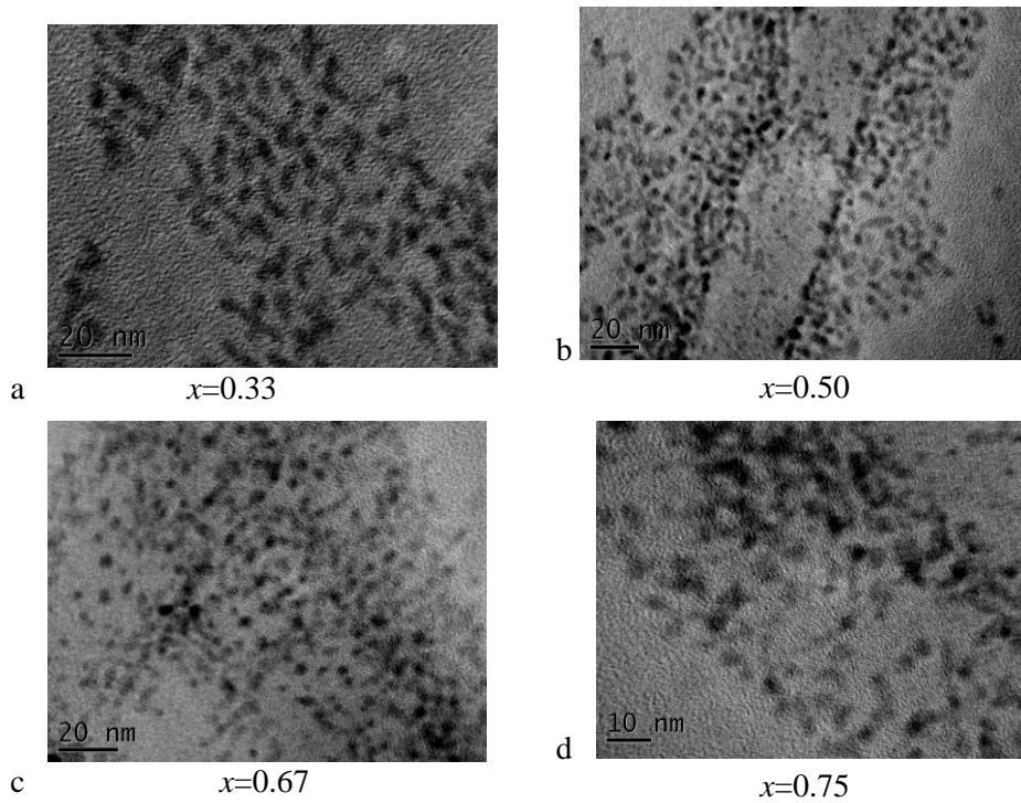
Fig. (5): HRTEM images of nano alloy CdSSe with different ratio S/(S+Se) = ((a) 0.33, (b) 0.5, (c) 0.67 and (d) 0.75) approximation of size 5.2nm.
