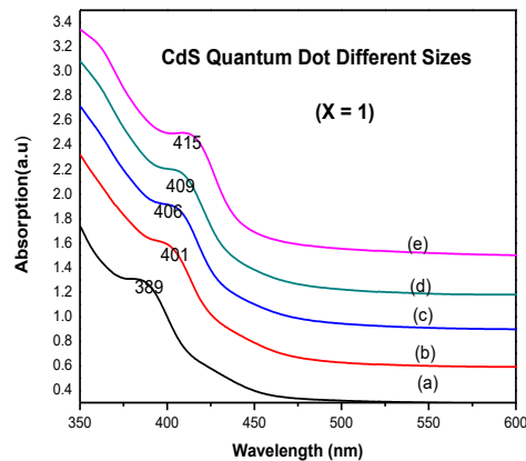
Fig. (1b). Absorption spectra for five samples of CdS QD labeled from (a) to (e).
