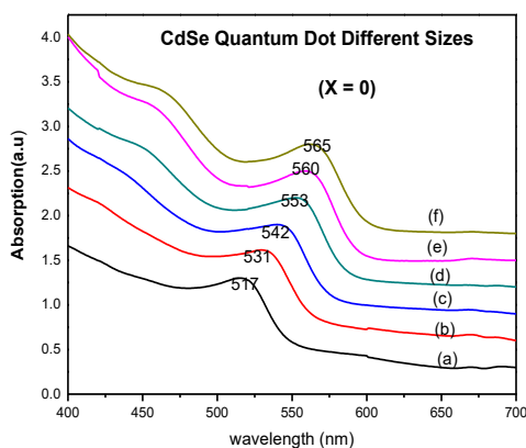
Fig. (1a). Absorption spectra for six samples of CdSe QD labeled from (a) to (f).
